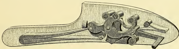
Modern Rebounding Gun-lock.
